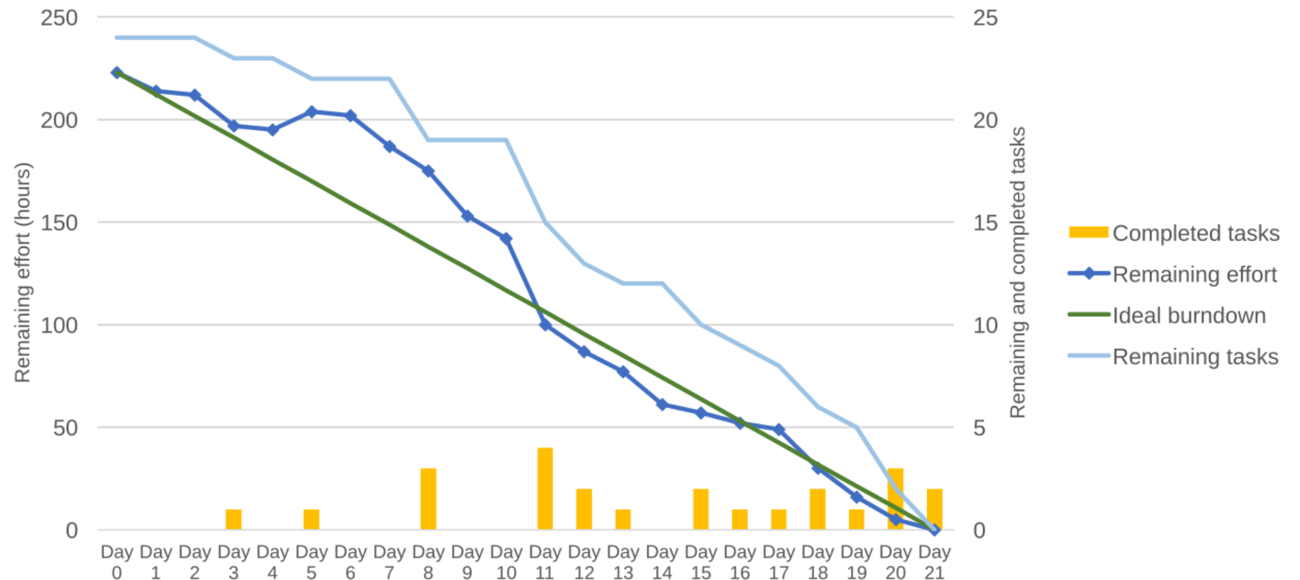
Sample Burndown Chart
